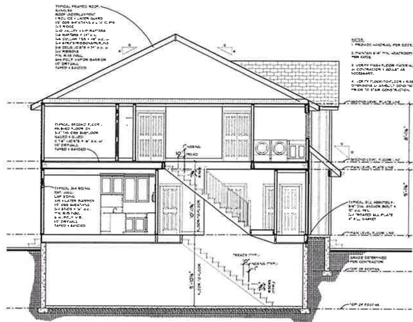
CROSS SECTION SCALE: 1/4" = 1'-0"
