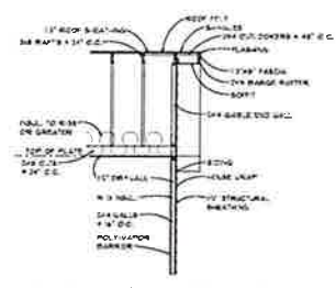
TYP. GABLE END SECTION SCALE: 1/4" = 1'-0"
