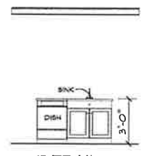
DETAIL 3 CABINET ELEVATIONS SCALE: 3/8" = 1'-0"
