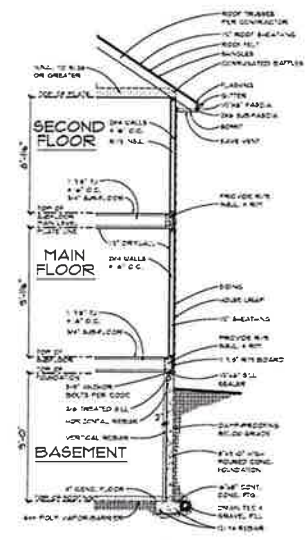
TYP. WALL SECTION SCALE: 1/4" = 1'-0"
